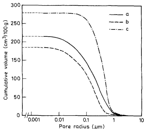
Figure 4. Pore size distribution curves for Wyoming montmorillonite saturated at 10 -3 M NaCl after: (a) Peldri II drying, (b) critical point drying, and (c) freeze drying.
