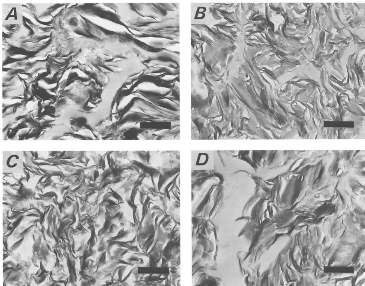
Figure 3. Transmission electron micrographs of ultrathin sections of Wyoming montmorillonite saturated at 1 M CaCl 2 after: (a) dehydration with acetone, (b) Peldri II drying, (c) critical point drying, and (d) freeze drying. Marker = 1 μm.
