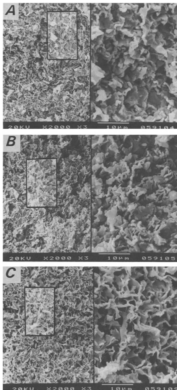
Figure 2. Scanning electron micrographs of Wyoming montmorillonite saturated at 10^{-3} M NaCl after: (a) Peldri II drying, (b) critical point drying, and (c) freeze drying.
