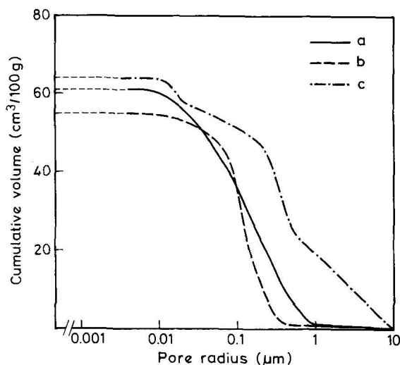
Figure 5. Pore size distribution curves for Wyoming montmorillonite saturated at 1 M CaCl 2 after: (a) Peldri II drying, (b) critical point drying, and (c) freeze drying.
