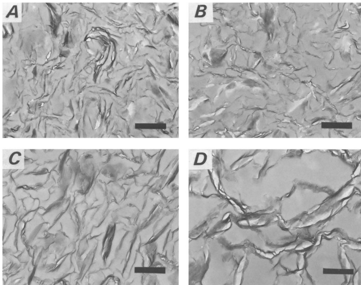
Figure 1. Transmission electron micrographs of ultrathin sections of Wyoming montmorillonite saturated at 10^{-3} M NaCl after: (a) dehydration with acetone, (b) Peldri II drying, (c) critical point drying, and (d) freeze drying. Marker = 1 \mu\text{m} .
