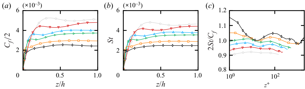
Figure 8. Distributions of local wall friction coefficient C_f = 2u_\tau^2/u_b^2 (a), local Stanton number St = (u_\tau \theta_\tau)/(u_b \theta_m) (b), and Reynolds analogy factor (c), along the left part of the lower wall. Symbols as in table 1.
