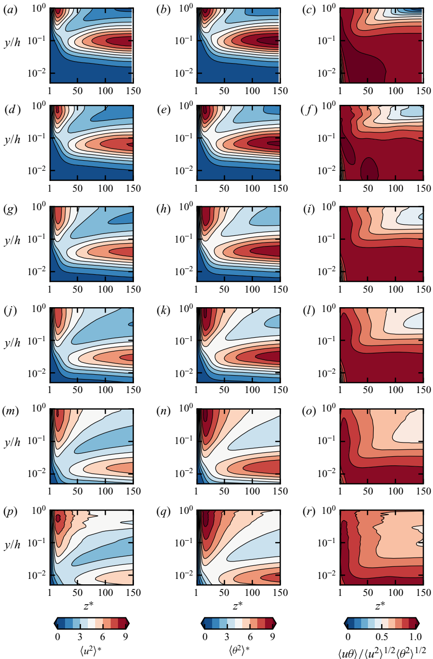
Figure 6. Streamwise velocity and temperature fluctuation intensities (in global inner units), and their correlation coefficient, in the proximity of a duct corner for flow cases A (a–c), B (d–f), C (g–i), D (j–l), E (m–o), F (p–r). Note that the horizontal coordinate ( z ) is given in inner units, and the vertical coordinate y is given in outer units and at a logarithmic scale.
