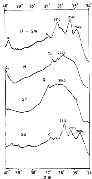
Figure 2. X-ray powder diffraction traces between 34^\circ and 40^\circ 2\theta of Li-bearing smectite having 0.21–0.50 Li/unit cell (Li-Sm), hectorite (H), stevensite (St), and saponite (Sa). Ca = calcite; Q = quartz; \text{CuK}\alpha radiation.
