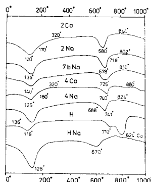
Figure 5. Differential thermal analysis curves of Li-bearing smectite samples and hectorite.
