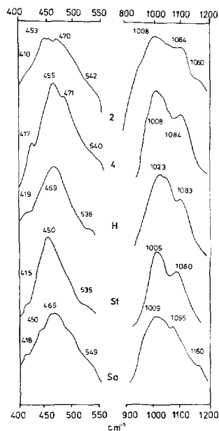
Figure 8. Infrared absorption spectra between 400–550 \text{cm}^{-1} and 900–1100 \text{cm}^{-1} of Li-bearing smectites, hectorite, stevensite, and saponite.
