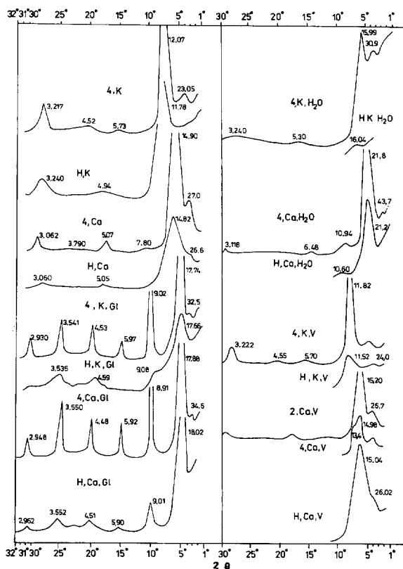
Figure 3. X-ray powder diffraction of Li-bearing smectite having 0.46 Li/unit cell (2), 0.21 Li/unit cell (4), and hectorite (H). Oriented aggregates, \text{CuK}\alpha radiation. Ca = Ca-saturated, Gl = glycerolated, \text{H}_2\text{O} = water treated, K = K-saturated, V = preserved in vacuum for two weeks in the presence of \text{CaCl}_2 .
