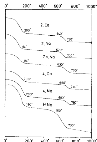
Figure 6. Thermogravimetric curves of Li-bearing smectite samples and hectorite.
