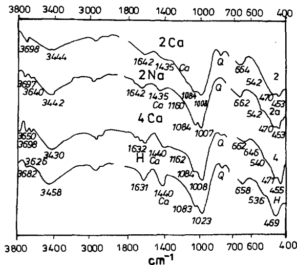
Figure 7. Infrared absorption spectra of Li-bearing smectite samples and hectorite.
