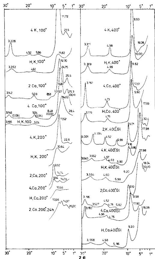
Figure 4. X-ray powder diffraction traces of Li-bearing smectites (samples 2 and 4) and hectorite (H), heated at different temperatures. Oriented aggregates, \text{CuK}\alpha radiation. K = K-saturated, Ca = Ca-saturated, 100° = analyzed 1 hr after heating for 2 hr at 100°C, 200° = analyzed 1 hr after heating for 2 hr at 200°C, 24 h = analyzed 24 hr after heating for 2 hr at 200°C, 400° = analyzed 1 hr after heating for 2 hr at 400°C, GI = glycerolated.
