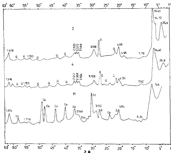
Figure 1. X-ray powder diffraction traces of Li-bearing smectites and hectorite. 2 = Li-bearing smectite having 0.46 Li/unit cell; 4 = Li-bearing smectite having 0.21 Li/unit cell; H = hectorite; Ca = calcite; Q = quartz; Dol = dolomite; CuK \alpha radiation.
