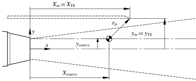
FIGURE 14. Sketch representation of an equivalent source located in the centre of the jet mixing layer (assumed to be the nozzle lip line), at a certain distance r_0 from a defined measurement point (plate trailing edge), for a given wavenumber.
