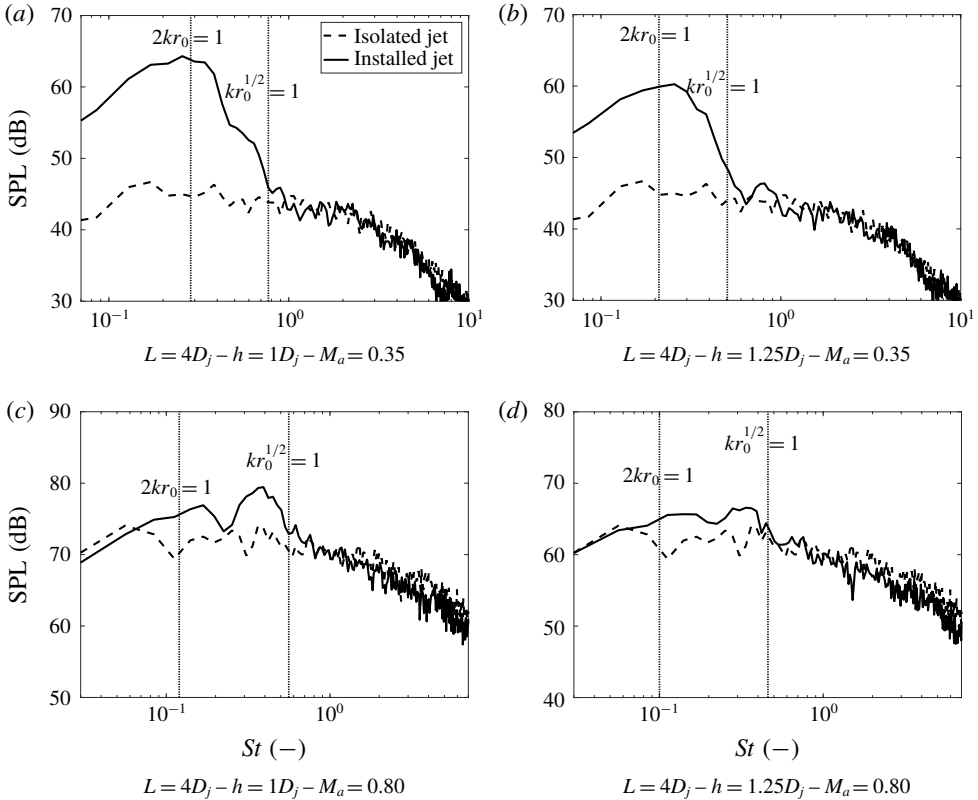
FIGURE 20. Far-field spectra with the frequency values where the compactness parameters 2kr_0 and kr_0^{1/2} are equal to 1, for Ma = 0.35 (a,b) and Ma = 0.80 (c,d). Spectra obtained for \theta = -90^\circ .
