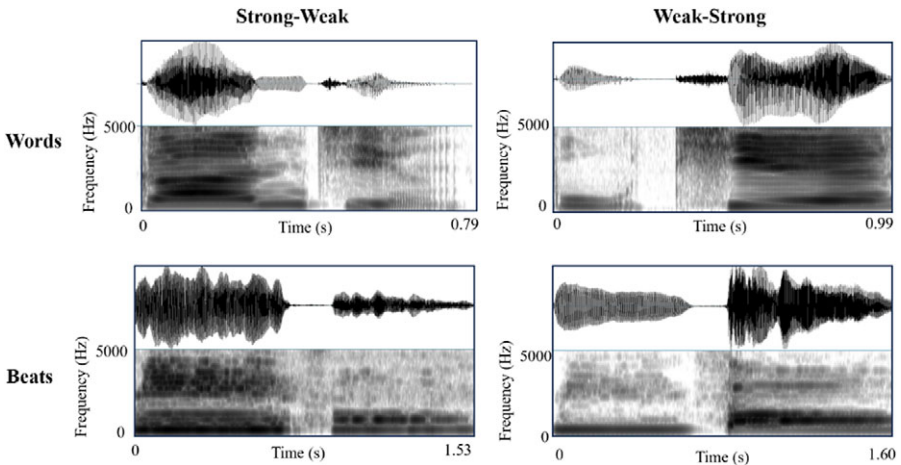
Figure 1. Oscillograms and spectrograms of the stimulus sample.
