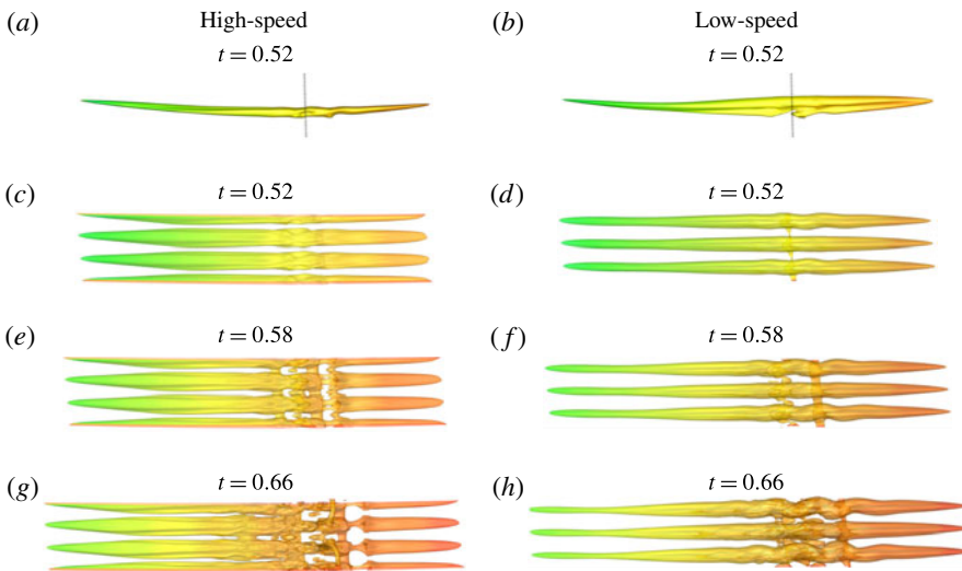
FIGURE 21. (Colour online) Iso-surfaces of streamwise perturbation velocity 0.05 ( a,c,e,g ) and -0.05 ( b,d,f,h ) at t = 0.52, 0.58 and 0.66 from top to bottom. The first row is lateral view with the dotted lines denoting x = 0.27 ; all the following rows are top view.
