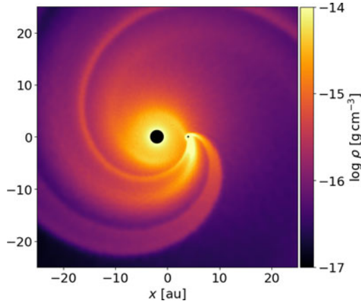
Figure 1. Density structure of a companion-perturbed AGB outflow, shown in a slice through the orbital plane with the AGB star on the left and the companion on the right; simulation from Esseldeurs et al. (2023) .
