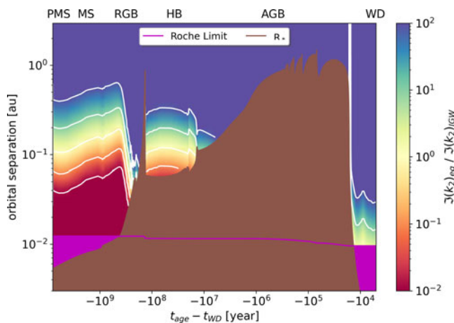
Figure 2. Competing dissipation strengths of the equilibrium ( \mathfrak{S}(k_2)_{eq} ) and dynamical ( \mathfrak{S}(k_2)_{IGW} ) tide as a function of the orbital separation and stellar age ( t_{age} upto the age where the star becomes a white dwarf t_{WD} ), for a 1.2 M_{\odot} host star; simulation from Esseledeurs et al. (in prep.).
