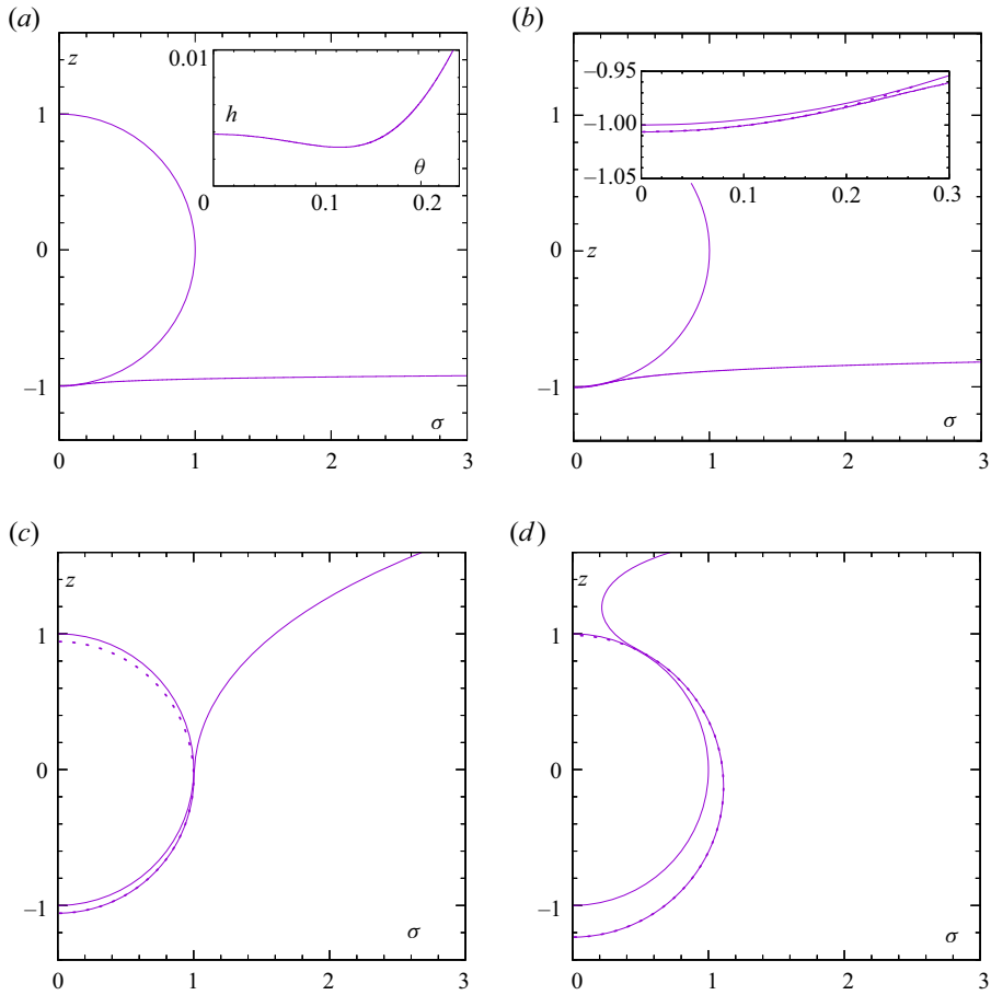
Figure 4. Interface profiles for JaCr = 10^{-8} and values of p_0 at, or to the right of, the maximum in figure 3(a): (a) p_0 = 2.4311 ( F/(JaCr)^{1/3} = 10.24 ), inset showing the local minimum in h ; (b) p_0 = 2.35 ( F/(JaCr)^{1/3} = 28.78 ), inset showing the spherical cap used to determine the contact angle \chi ; (c) p_0 = 2.0 ( F/(JaCr)^{1/3} = 464.1 ); and (d) p_0 = 1.8 . Solid curves, numerical solution of (3.3). Broken curves, sphere osculating with the interface at its lowest point.
