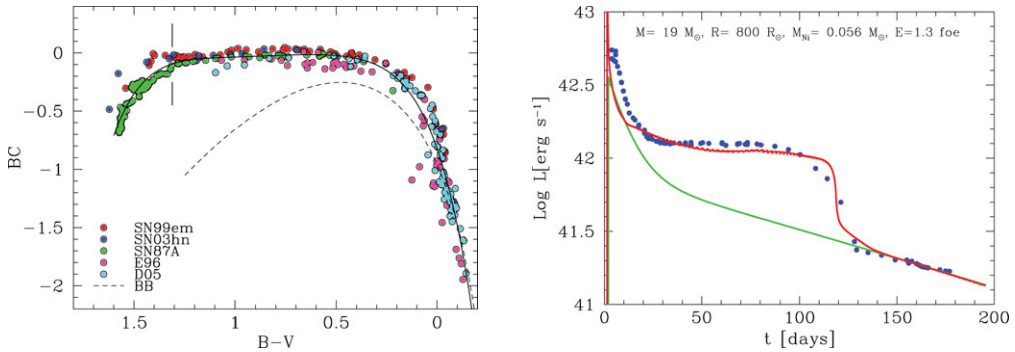
Figure 7. Hydrodynamical models for TypeII-P SN Light Curves. Left: Bolometric correction versus B-V. Right: Light curve for SNeII-P
