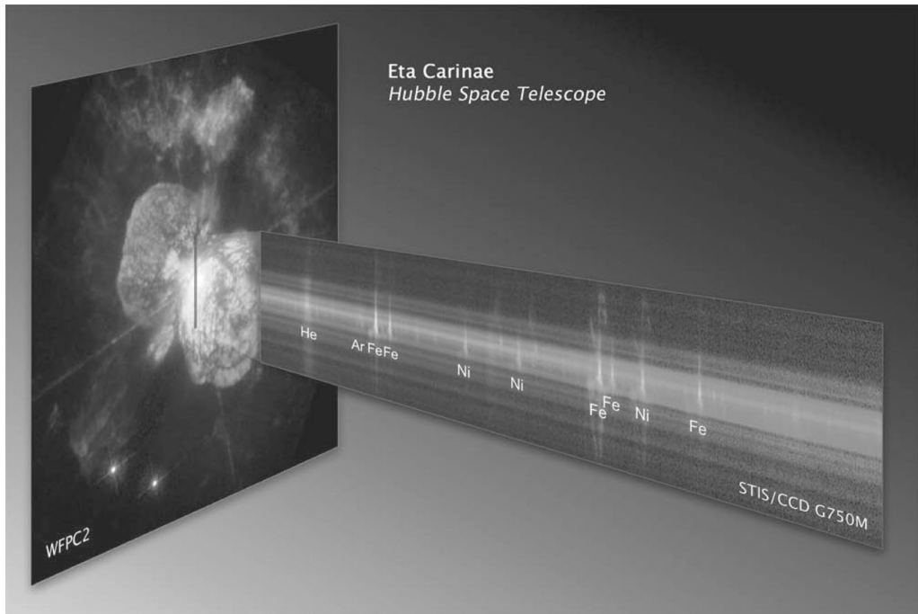
Figure 2. An example of what is so intriguing about \eta Car: the extended wind and ejecta. A 0.1'' -wide slit of the Hubble Space Telescope Imaging Spectrograph samples the extended structure surrounding \eta Car as imaged by Hubble Space Telescope. Continuum and broad line emission at the center of the spectrum originate from the extended interacting winds. Narrow forbidden emission lines shifted with velocities up to 500 \text{ km s}^{-1} come from the interior of the Homunculus, thrown out in the 1840s. An estimated 10 to 20 M_{\odot} was ejected during the Great Eruption as well as up to 0.5 M_{\odot} in the lesser eruption of the 1890s. How did the ejecting star survive and what clues does this provide us on the late stages of massive stellar evolution? (Image courtesy of NASA and STScI)
