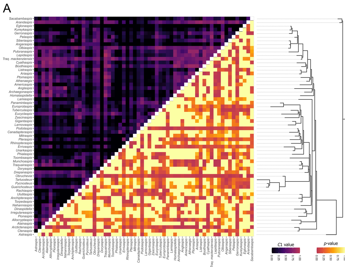
Figure 5. Quantifying convergence in headshield processes of Pteraspidomorphi through Stayton's (A) C1 and (B) Ct1 metrics. The Stayton's C1 and Ct1 metrics, depicted in purple, provide a measure of convergence strength, while the accompanying p -values, shown in yellow-orange, indicate the statistical significance of the observed convergence. Note that instances where Ct1 metrics and p -values are displayed in white result from uninformative analyses, typically due to comparisons between sister taxa or taxa lacking contemporaneous ancestral nodes. The phylogenetic tree is based on Randle et al. (2022), Glinnskiy (2018), Dec (2019b), and Janvier (1996).
