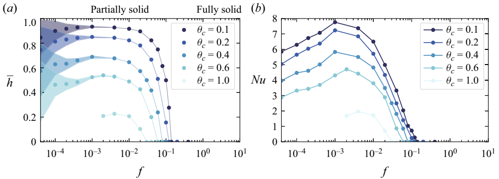
Figure 7. (a) Mean equilibrium solid–liquid interface height \bar{h} as a function of the modulation frequency f at different \theta_c . The shaded regions represent the region between the maximum height and minimum height of the solid–liquid interface during one period. Two regimes are classified: ‘fully solid’ and ‘partially solid’ as f decreases. (b) Plots of Nu at the bottom plate as a function of the modulation frequency f at different \theta_c . Here, Nu is calculated based on (2.7). In all cases, Nu(f) shows a pronounced maximum at medium frequencies.
