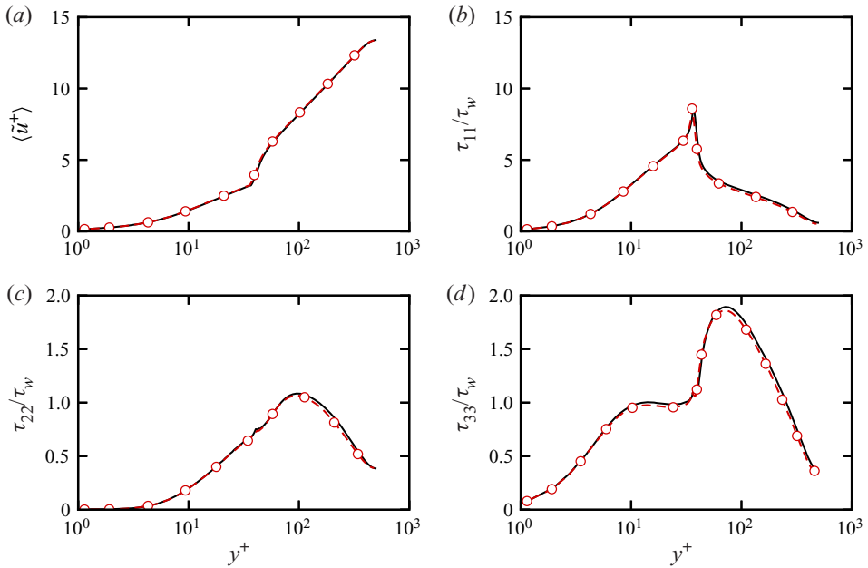
Figure 16. Mesh refinement study for turbulent channel flow over cubic roughness at bulk Mach number M_b = 0.2 and bulk Reynolds number Re_b = 10293 . Flow case M02A (solid line) has N_x \times N_y \times N_z = 3088 \times 384 \times 1536 mesh points and case M02B (circles) N_x \times N_y \times N_z = 4096 \times 384 \times 2048 mesh points, corresponding to 40 and 60 grid points per roughness element, respectively.
