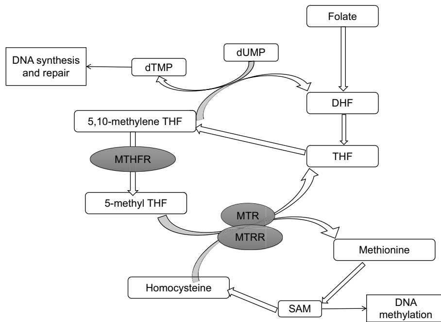
Fig. 1. Overview of folate-mediated one-carbon metabolism (OCM) and related enzymes. 5,10-methylene THF, 5,10-methylenetetrahydrofolate; 5-methyl-THF, 5-methyltetrahydrofolate; DHF, dihydrofolate; dTMP, deoxythymidine; MTHFR, methylenetetrahydrofolate reductase; MTR, 5-methyltetrahydrofolate-homocysteine methyltransferase reductase; MTRR, 5-methyltetrahydrofolate-homocysteine methyltransferase reductase; SAM, S-adenosylmethionine; THF, tetrahydrofolate.
