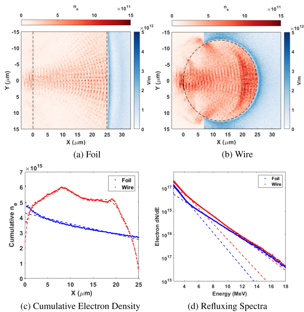
Figure 6. Results from PIC simulations. (a) Electron density (red scale) and E -field (blue scale) spatial maps for the foil simulation at 500 fs. (b) Same as (a) but for wire simulation. (c) Cumulative on-axis electron density over the entire simulation. 0 \mu\text{m} indicates front surface for each target. (d) Refluxing electron spectra with a two-temperature distribution, see Table 1 for values.
