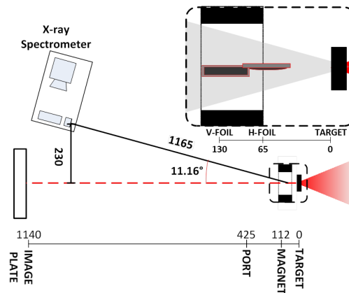
Figure 2. Schematic of the primary imaging diagnostics. Main image shows the emission line, with penumbral foils and hard X-ray spectrometers included. The inset is an expansion of the penumbral foil setup, and the grey cone represents the forward X-ray emission from target, with all distances in mm measured from target position.
