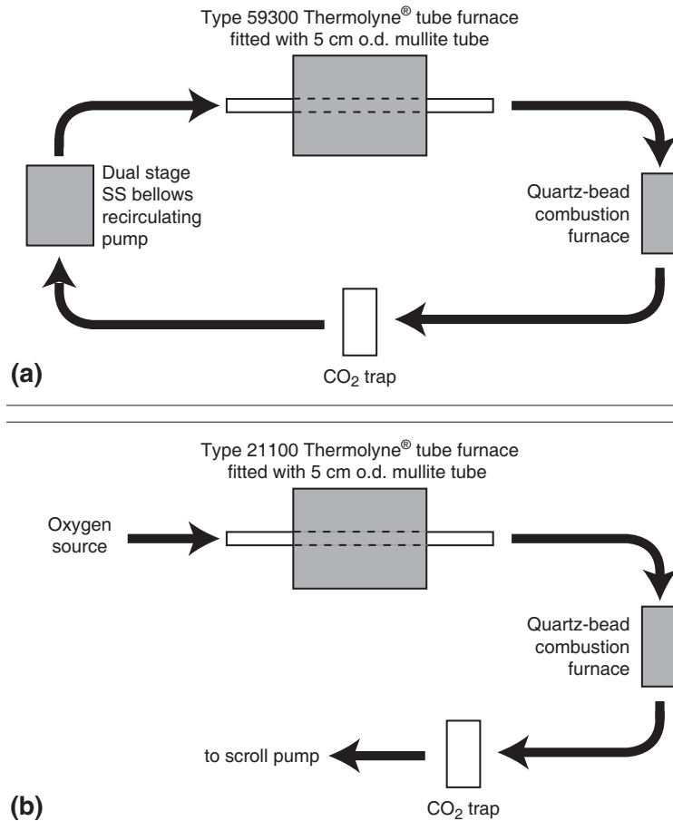
Figure 1 Schematic diagrams of (a) the original in situ 14 C extraction line (after Lifton et al. 2001) and (b) the modified extraction line in our laboratory at the University of Arizona. Dark arrows show the flow path of O 2 carrier gas, which is kept at pressures equivalent to ~6.7 kPa at 170 °C. Carbon species liberated from a sample are fully oxidized to CO 2 in the quartz-bead furnace and collected in the CO 2 trap. Contaminant gases are subsequently removed, the sample CO 2 is diluted with 14 C-free CO 2 , and converted to graphite for analysis by AMS.
