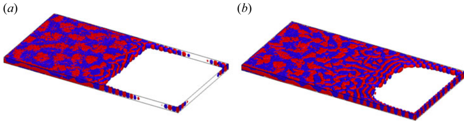
Figure 13. Isosurfaces of u_z = 0.01 (red) and u_z = -0.01 (blue) for (a) \delta = 1 and (b) \delta = 9 . In the regions with strong magnetic fields, convective motions are confined near the sidewalls.
