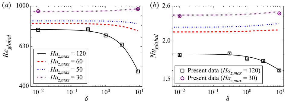
Figure 12. Plots versus \delta of (a) the global Reynolds number Re_{global} (black squares for Ha_{z,max} = 120 and purple circles for Ha_{z,max} = 30 ), computed from our numerical data using (2.12), and (b) the global Nusselt number Nu_{global} (black squares for Ha_{z,max} = 120 and purple circles for Ha_{z,max} = 30 ), computed from our numerical data using (2.13). Also shown in the plots are the estimates (solid curves) of Re_{global} and Nu_{global} computed using (3.14) and (3.15) for different values of Ha_{z,max} .
