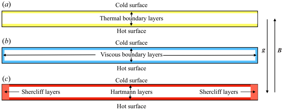
Figure 3. Sketches of the vertical ( x - z ) cross-section of a Rayleigh–Bénard convection cell (with aspect ratio similar to ours) under a vertical magnetic field, showing (a) thermal boundary layers, (b) viscous boundary layers, and (c) Hartmann and Shercliff layers.
