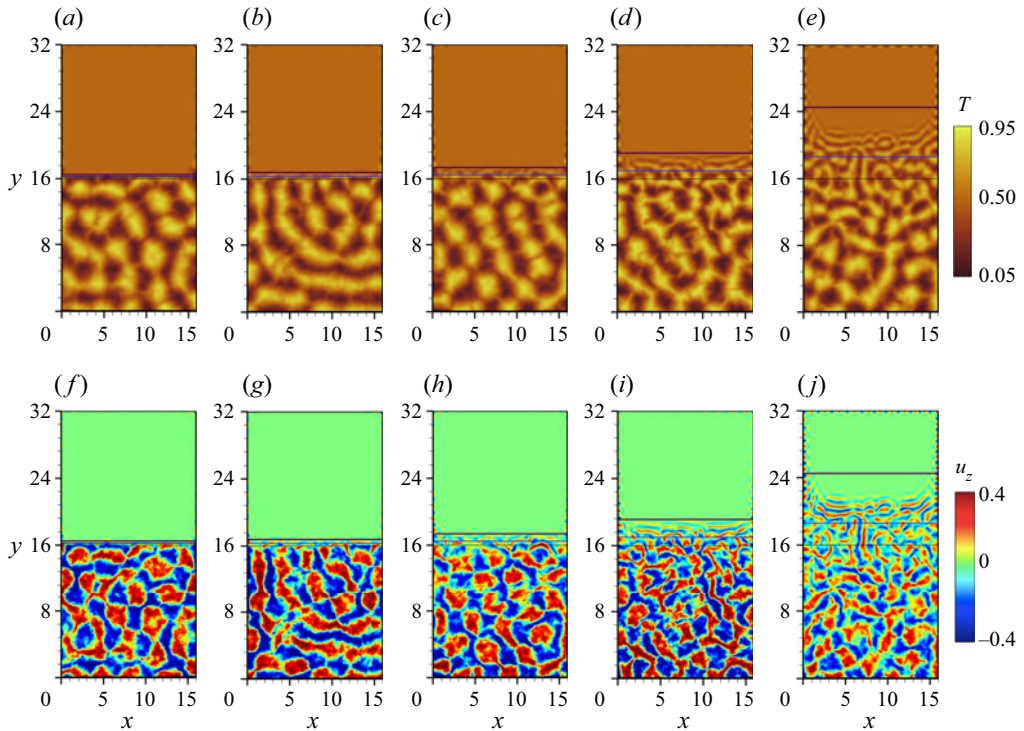
Figure 4. Contour plots of time-averaged fields on the horizontal midplane for different fringe widths of the imposed magnetic field. Plots of the temperature field for (a) \delta = 0.01 , (b) \delta = 0.3 , (c) \delta = 1 , (d) \delta = 3 , and (e) \delta = 9 . Plots of the vertical velocity field for (f) \delta = 0.01 , (g) \delta = 0.3 , (h) \delta = 1 , (i) \delta = 3 , and (j) \delta = 9 . The flows are organized into large-scale patterns that extend over scales larger than the domain height. The positions corresponding to Ha_z(y) = Ha_{z,c} , Ha_z(y) = 0.8Ha_{z,c} , and the edge of the magnetic poles are represented by purple, blue and black horizontal lines, respectively, in decreasing order of thickness. The magnetic poles extend from y = 16 to y = \infty .
