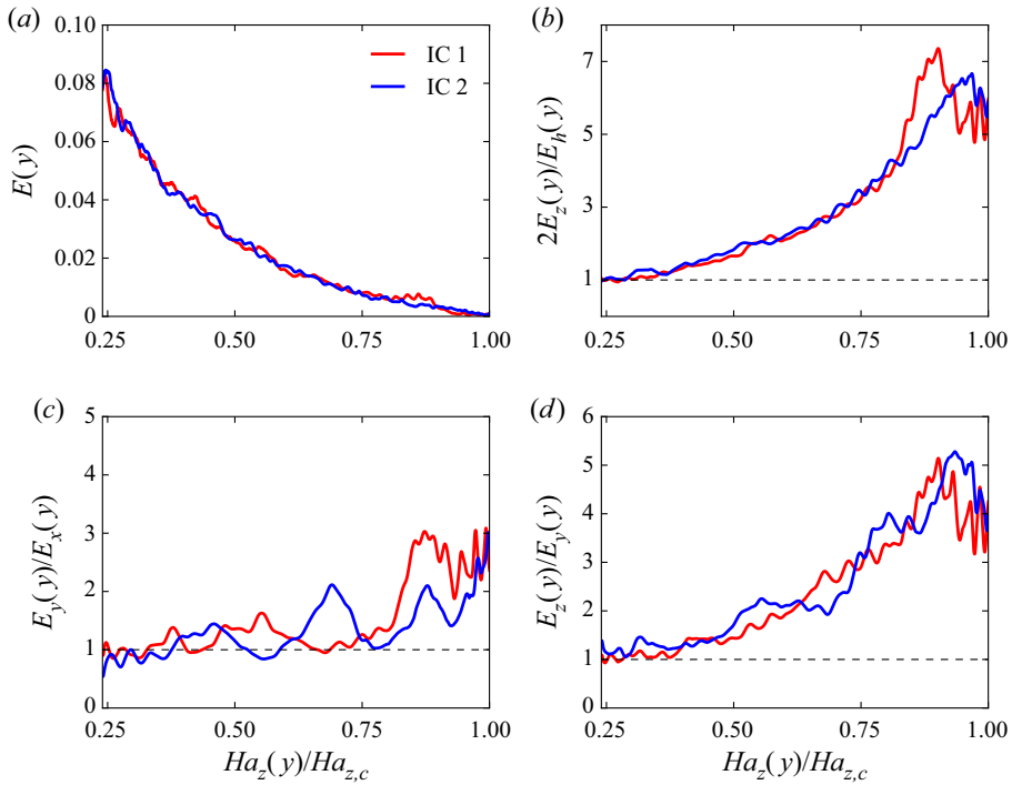
Figure 17. For \delta = 9 and different initial conditions: mean profiles of (a) the local kinetic energy E(y) , (b) the local vertical anisotropy parameter 2E_z(y)/E_h(y) , (c) the local horizontal anisotropy parameter E_y(y)/E_x(y) , and (d) the ratio of the kinetic energy along the z - and y -directions, versus the Hartmann number, Ha_z(y) , based on the mean vertical magnetic field B_z(y) . For both sets of initial conditions, the variations of E(y) with Ha_z(y) are identical, and the anisotropy parameters increase with the local vertical magnetic field strength.
