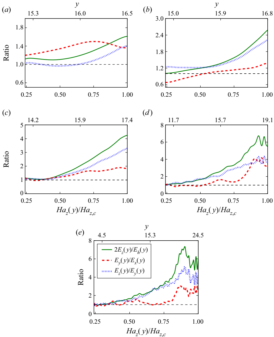
Figure 8. Mean profiles of the local vertical anisotropy parameter 2E_z(y)/E_h(y) (solid green curves), the local horizontal anisotropy parameter E_y(y)/E_x(y) (dashed red curves), and the ratio of the kinetic energy along the z - and y -directions E_z(y)/E_y(y) (dotted blue curves), versus the normalized Hartmann number Ha_z(y)/Ha_{z,c} based on the mean vertical magnetic field B_z(y) , for (a) \delta = 0.01 , (b) \delta = 0.3 , (c) \delta = 1 , (d) \delta = 3 , and (e) \delta = 9 . Both the vertical and horizontal anisotropy parameters increase with the local vertical magnetic field strength.
