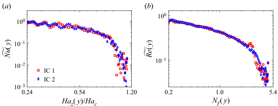
Figure 18. Variations of the normalized local planar Nusselt and Reynolds numbers with the normalized local vertical magnetic field strengths. For IC 1 and IC 2: (a) normalized local Nusselt number \tilde{Nu}(y) versus the normalized local Hartmann number Ha_z(y)/Ha_c , based on vertical magnetic field strength; and (b) normalized local Reynolds number \tilde{Re}(y) versus the local free-fall interaction parameter N_f(y) .
