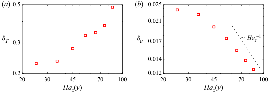
Figure 11. Boundary analysis for \delta = 9 : (a) local thermal boundary layer thickness \delta_T(y) , and (b) local viscous boundary layer thickness \delta_u(y) , near the top and bottom walls, versus the local Hartmann number Ha_z(y) . The thermal boundary layer thickness increases with the increase of Ha_z(y) . The viscous boundary layer thickness decreases with increasing Ha_z(y) and approaches the Hartmann-type scaling \delta_u \sim Ha_z^{-1} at large Hartmann numbers.
