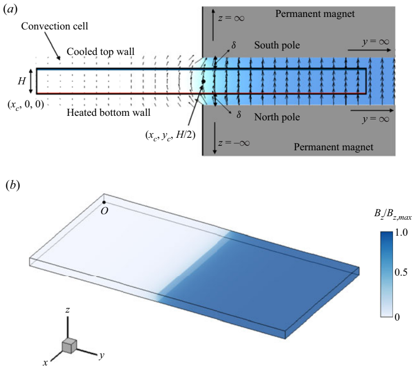
Figure 1. (a) Schematic of the vertical section at x = x_c = l_x/2 of the proposed magnetoconvection arrangement. The semi-infinite permanent magnets (in grey) generate the localized magnetic field represented by the vector plots drawn in the convection cell. The magnetic field distribution is described by (2.1)–(2.3). (b) A three-dimensional view of the convection cell used in our study, with the density contours of the vertical component of the normalized imposed magnetic field for \delta/H = 0.01 . Here, O refers to the point at the origin, and \delta is the gap between the magnetic pole and the convection cell.
