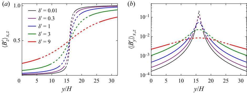
Figure 2. Distribution of the profiles of (a) vertical magnetic field and (b) absolute value of the horizontal magnetic field, both averaged over x and z , along the lengthwise direction (normalized by the height H of the cell) for different values of the normalized gap ( \delta' = \delta/H ) between the magnetic poles and the thermal plates. The magnetic fields are normalized by the maximum value of the vertical magnetic field ( B_z' = B_z/B_{z,max} and B_y' = B_y/B_{z,max} ). The curves are represented as dashed lines in the fringe zone, and as solid lines outside the fringe zone.
