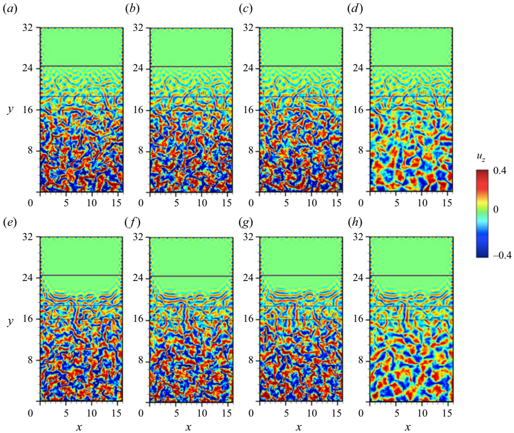
Figure 16. Contour plots of vertical velocity u_z for \delta = 9 in the horizontal midplane for different initial conditions. For the simulation IC 2, contour plots of u_z at (a) t = 0 , (b) t = 9 , and (c) t = 18 , where t is measured from the time stamp of the first snapshot saved at statistically steady state. For the simulation IC 1, contour plots of u_z at (e) t = 0 , (f) t = 9 , and (g) t = 18 , where t is measured from the time stamp of the first snapshot saved at statistically steady state. Contour plots of time-averaged vertical velocity for (d) IC 2 and (h) IC 1. The positions corresponding to Ha_z(y) = Ha_{z,c} , Ha_z(y) = 0.8Ha_{z,c} and the edge of the magnetic poles are represented by purple, blue and black horizontal lines, respectively, in decreasing order of thickness. The magnetic poles extend from y = 16 to y = \infty .
