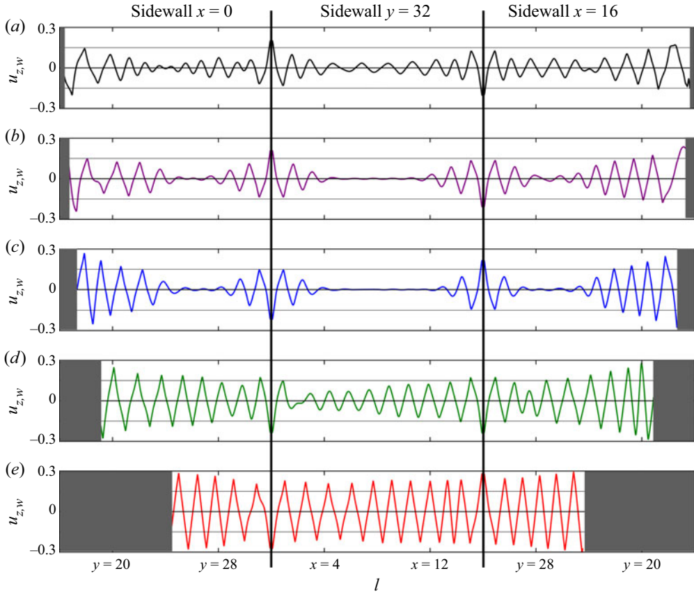
Figure 15. Vertical velocity u_{z,w} measured on the horizontal midplane at distance \bar{\delta}_w from the sidewalls in the regions Ha(y) > Ha_{z,c} (non-shaded regions) for (a) \delta = 0.01 (black curve), (b) \delta = 0.3 (purple curve), (c) \delta = 1 (blue curve), (d) \delta = 3 (green curve), and (e) \delta = 9 (red curve). The shaded regions correspond to Ha_z(y) < Ha_{z,c} , where the flow is not fully suppressed in the bulk. The amplitudes of the wall modes in the regions away from the corners exhibit a non-monotonic dependence on \delta . Note that these plots are resolved by a total of at least 9000 grid points in the horizontal direction.
