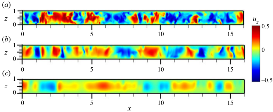
Figure 6. Contour plots of the time-averaged vertical velocity field for \delta = 9 in vertical planes at (a) y = 3.4 ( Ha_z(y) = 25 ), (b) y = 11.9 ( Ha_z(y) = 45 ), and (c) y = 19.7 ( Ha_z(y) = 75 ). The velocity fluctuations decrease with the increasing magnetic field strength along y .
