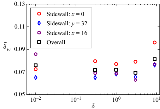
Figure 14. The average distance between the wall modes and the sidewalls versus \delta in the regions Ha_z(y) > Ha_{z,c} . The wall modes are more attached to the lateral sidewalls than to the longitudinal sidewalls.
