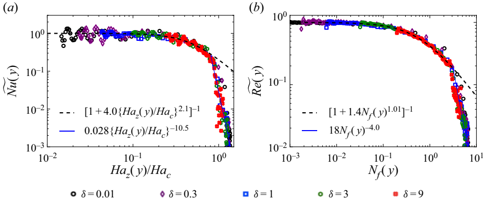
Figure 10. Variations of the normalized local Nusselt and Reynolds numbers with the normalized local vertical magnetic field strengths. For \delta = 0.01-9 : (a) normalized local Nusselt number \tilde{Nu}(y) versus the normalized local Hartmann number Ha_z(y)/Ha_c , based on vertical magnetic field strength; and (b) normalized local Reynolds number \tilde{Re}(y) versus the local free-fall interaction parameter N_f(y) . The best-fit curves for the above data are also shown.
