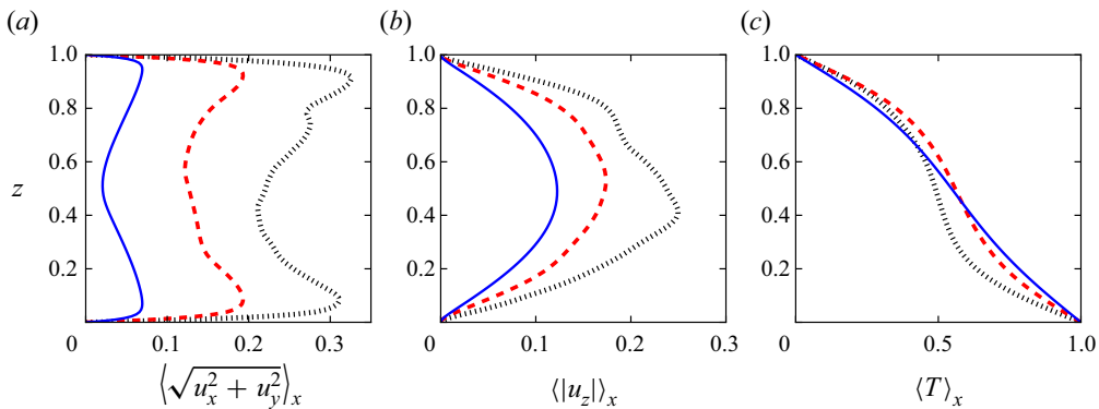
Figure 7. Profiles for \delta = 9 of (a) the mean horizontal velocity \langle \sqrt{u_x^2 + u_y^2} \rangle_x , (b) the mean absolute vertical velocity \langle |u_z| \rangle_x , and (c) the mean temperature \langle T \rangle_x along the vertical z -direction, at y = 3.4 (black dotted curves), y = 11.9 (red dashed curves), and y = 19.7 (blue solid curves). As the magnetic field strength increases along y , the velocity fluctuations decrease and the temperature approaches the linear conduction profile.
