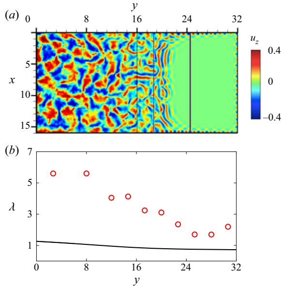
Figure 5. Pattern analysis for \delta = 9 . (a) Contour plot of the time-averaged vertical velocity field on the horizontal midplane. Solid lines are replotted from figure 4. (b) The evolution of the characteristic horizontal length scale of the superstructures (red circles) and the critical wavelength \lambda_c (black curve) at the onset of convection along the horizontal y -direction. The length scale of the convection patterns becomes smaller along the direction of the increasing magnetic field, and is larger than the critical wavelength.
