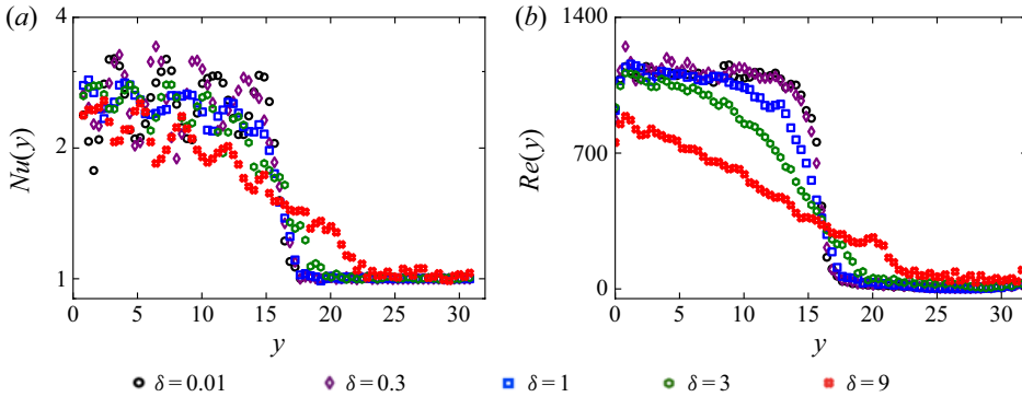
Figure 9. Variations of the local planar Nusselt and Reynolds numbers with the longitudinal direction y . For \delta = 0.01-9 : (a) local Nusselt number Nu(y) , and (b) local Reynolds number Re(y) , versus y .
