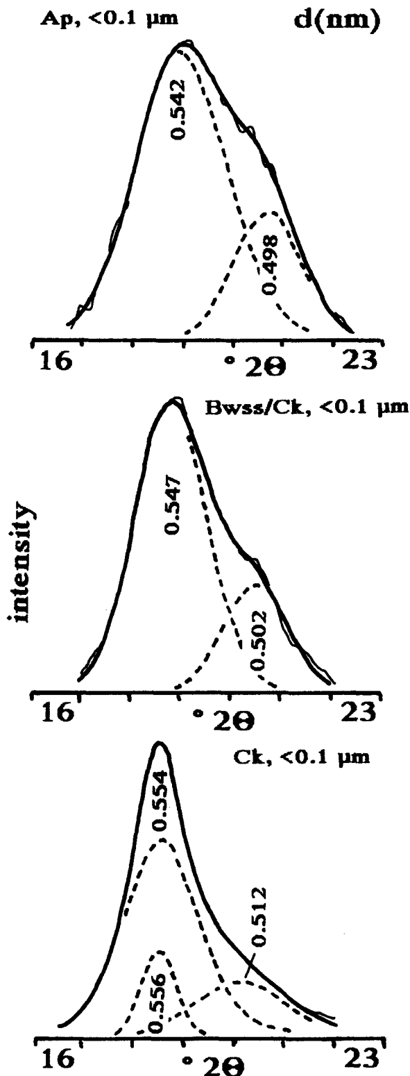
Figure 4. Decomposed XRD patterns in the 16–23 2\theta region. —: experimental curve, ---: elementary computed curve, —·—: best fit computed curve. Ca-saturated, ethylene glycol solvated. \text{CoK}\alpha radiation.
