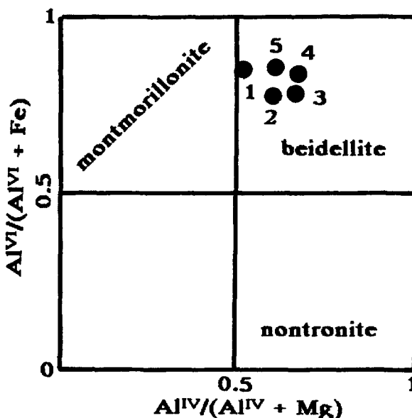
Figure 10. Octahedral composition and relative tetrahedral charge of the fine clay (<0.1 \mu\text{m} ) samples. 1: Ck, 2: Bwss/Ck, 3: Bwss2, 4: Bwss1, 5: Ap.
