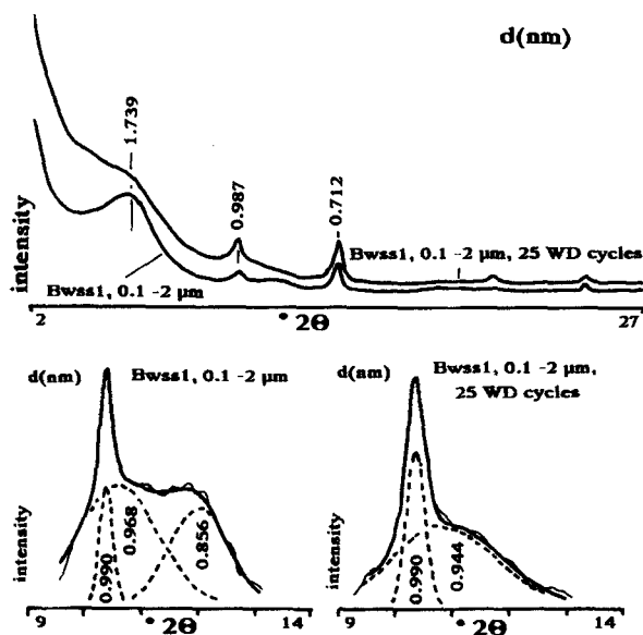
Figure 7. XRD patterns from the untreated and 25 WD cycles treated Bwss1, 0.1–2 \mu\text{m} samples. Ca-saturated, ethylene glycol solvated. \text{CoK}\alpha radiation.
