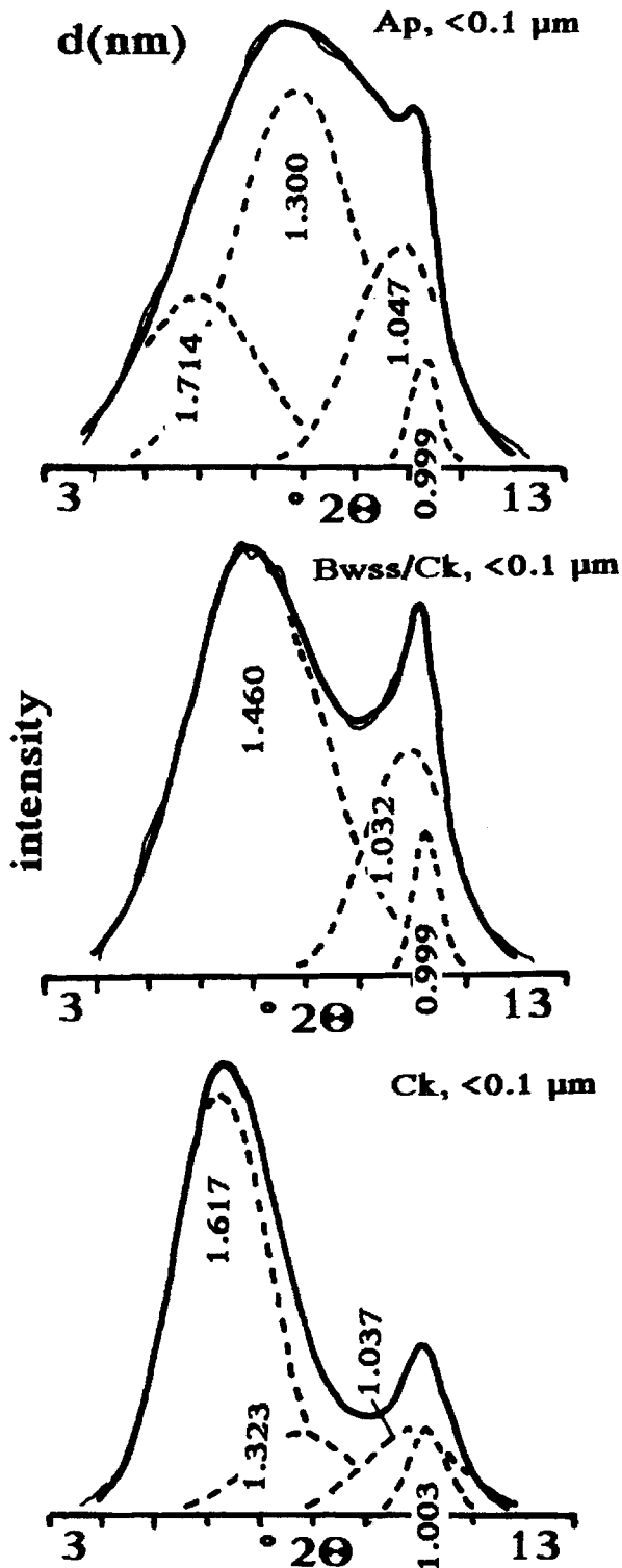
Figure 5. Decomposed XRD patterns in the 3–13 ^{\circ}2\theta region. —: experimental curve, ---: elementary computed curve, —: best fit computed curve. K-saturated, heated to 200 ^{\circ}\text{C} , ethylene glycol solvated. \text{CoK}\alpha radiation.
