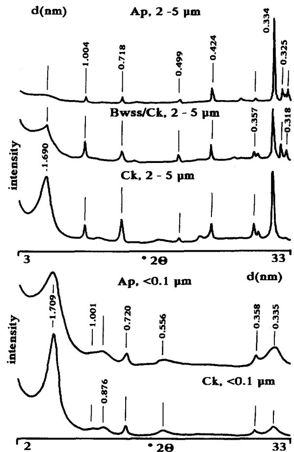
Figure 2. XRD patterns for fine silt (2–5 \mu m) and fine clay (<0.1 \mu m) subfractions. Ca-saturated, ethylene glycol solvated. CoK \alpha radiation.
