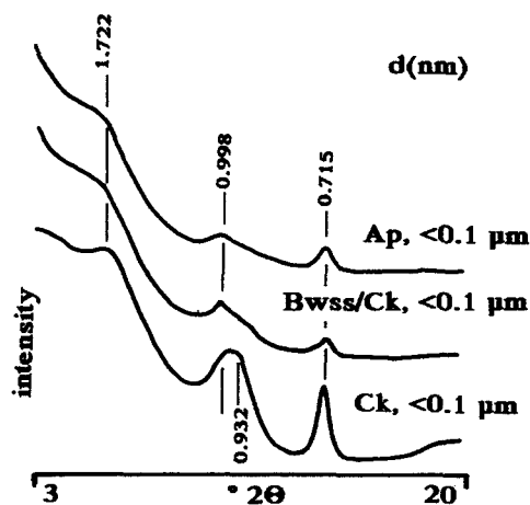
Figure 3. XRD patterns for fine clay subfractions. Li-saturated, heated to 300°C, ethylene glycol solvated. \text{CoK}\alpha radiation.
