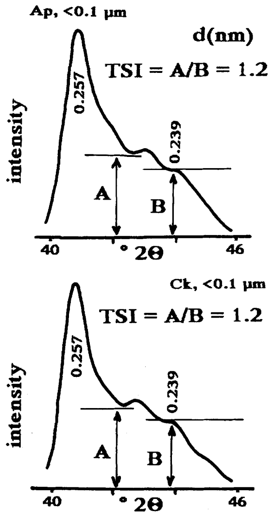
Figure 6. XRD patterns from randomly oriented powders. \text{CoK}\alpha radiation. Definition and computation of TSI, the turbostratic index (see Reynolds 1992).
