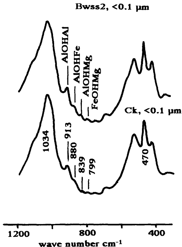
Figure 9. FTIR spectra for the Bwss2, <0.1 \mu\text{m} and Ck, <0.1 \mu\text{m} samples.
