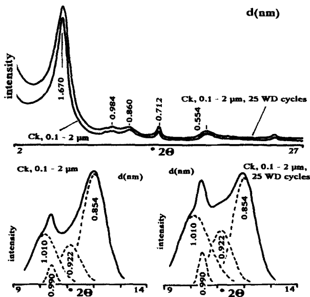
Figure 8. XRD patterns from the untreated and 25 WD cycles treated Ck, 0.1–2 \mu\text{m} samples. Ca-saturated, ethylene glycol solvated. \text{CoK}\alpha radiation.
