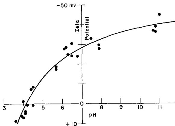
Fig. 6. Zeta potential of sodium kaolinite.
