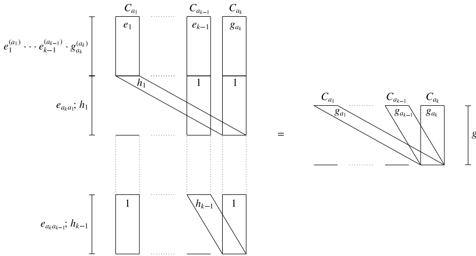
FIGURE 4. Diagrammatic proof that g = e_1^{(a_1)} \cdots e_{k-1}^{(a_{k-1})} \cdot g_{a_k}^{(a_k)} \cdot e_{a_k a_i; h_1} \cdots e_{a_k a_{i-1}; h_{k-1}} .
