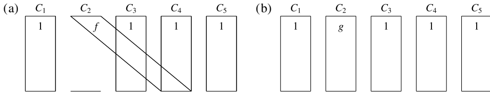
FIGURE 3. Diagrammatic representation of (a) e_{42;f} and (b) g^{(2)} from \mathcal{T}(X, \mathcal{P}) with m = 5 .
