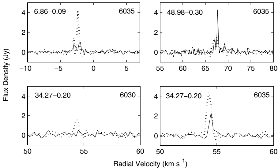
Figure 1. Spectra of new OH masers at the 6030- and 6035-MHz transitions. LCP and RCP are displayed as dashed and solid lines, respectively. The channel resolution is 0.2 km s -1 and the beamsize is approximately 3 arcminutes.
