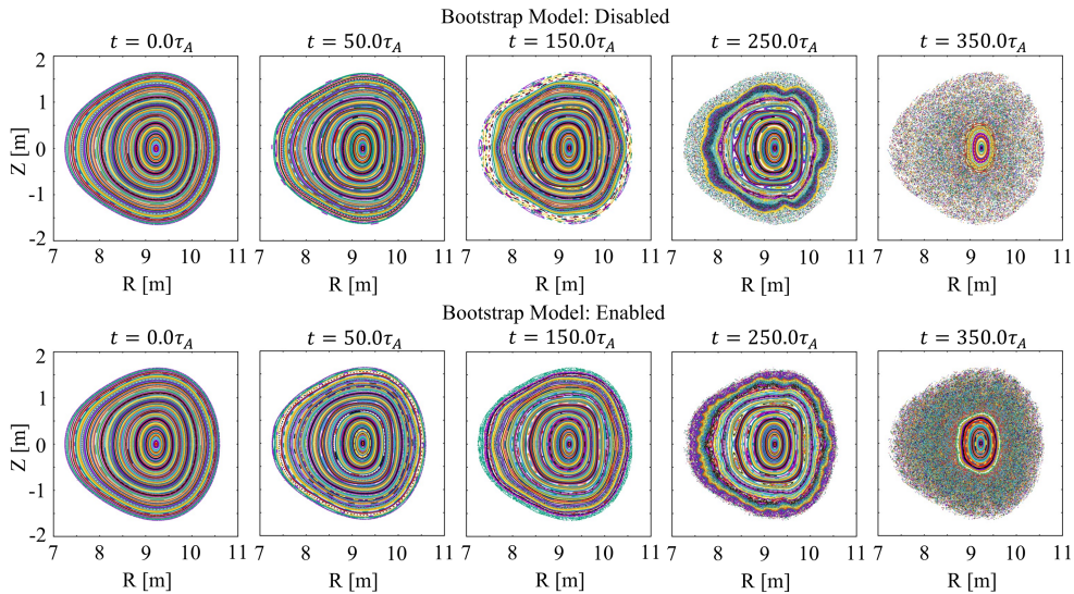
FIGURE 6. Poincaré sections of the magnetic field starting from a QA stellarator equilibrium optimized at 2.5 % plasma beta for the case with resistivity scale factor \eta_0 = 10^4 (QA_Case2). The sections are shown as a function of time for 0 \leq t \leq 350\tau_A , comparing simulations with the bootstrap model disabled (top row) and enabled (bottom row).
