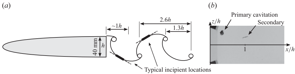
Figure 5. (a) Schematic of the von Kármán wake of the bluff hydrofoil showing preferential inception locations. (b) Image from a high-speed video of concurrent inception in primary and secondary vortices.
