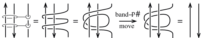
Figure 23: A band-# move realizes \tau_{ij}^2 .
