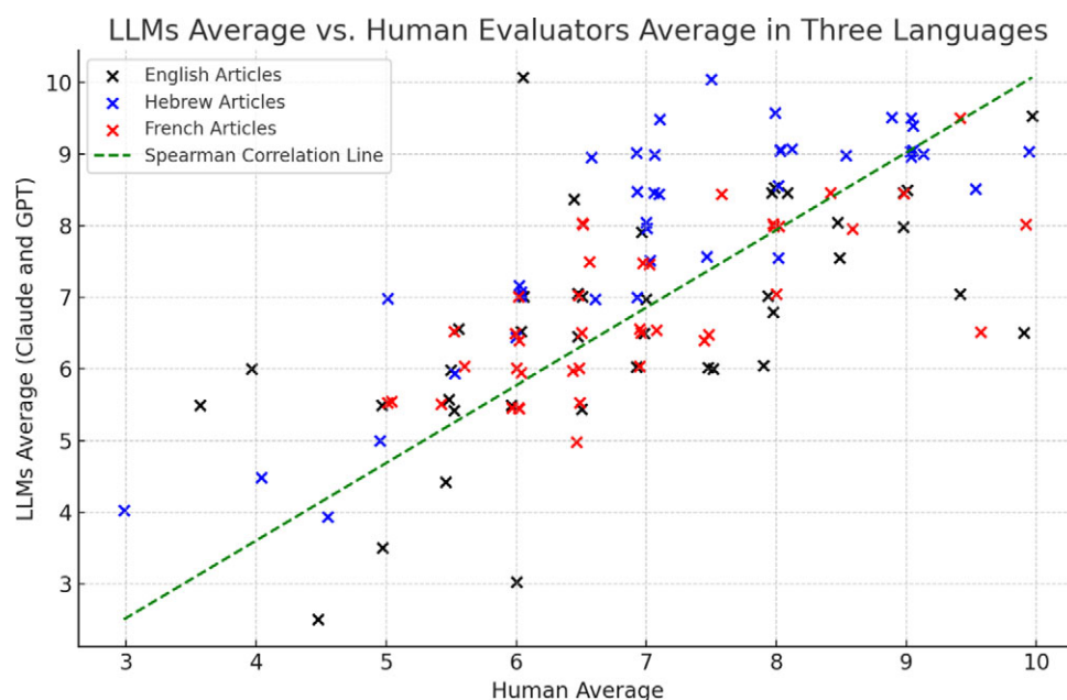
Figure 1. Average evaluations of large language models (LLMs) with human evaluators across three languages: English (black × marks), Hebrew (blue × marks), and French (red × marks).
