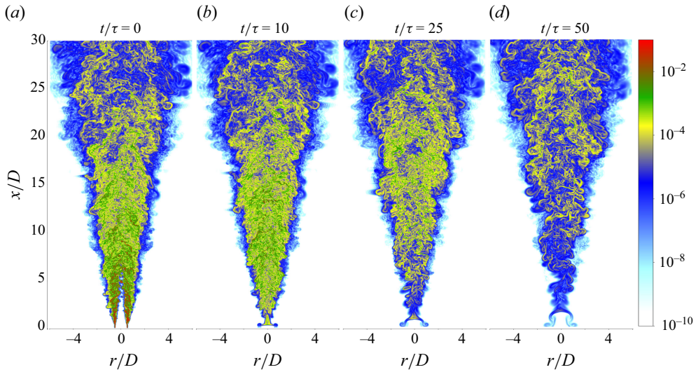
Figure 4. Non-dimensional instantaneous SDR in (a) the steady-state jet, and the stopping jet at times after stopping (b) 10\tau , (c) 25\tau , (d) 50\tau .
