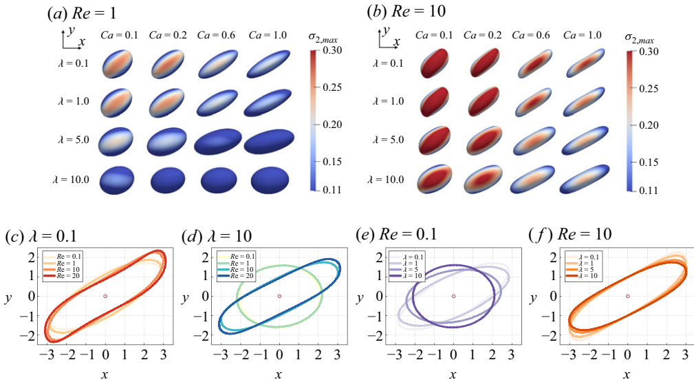
Figure 4. Deformation of capsules in the simple shear flow on the x – y plane across the capsule centroid in the cases (a) Re = 1 and (b) Re = 10 . The capsules are coloured with the maximum elastic stress \sigma_{2,max} on its surface when the flow is fully developed. Capsule outlines on the cut plane x – y across the capsule centroid highlighted with pink dot showing (c–d) effects of Re on the capsules at \lambda = 0.1 and 1; (e–f) effects of \lambda on the capsules at Re = 0.1 and 10.
